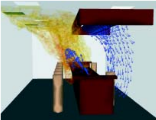
CFD simulation of smoke concentration in the bar
