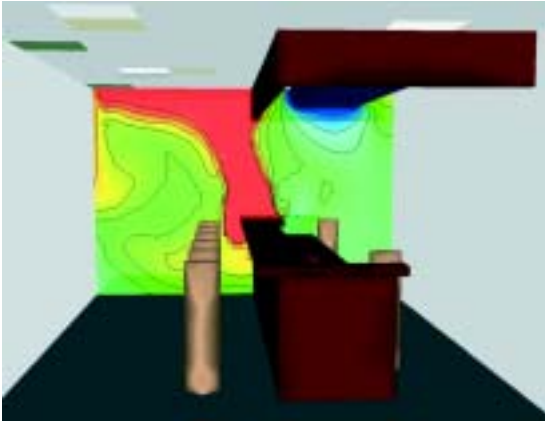
Flow simulation of a bar
